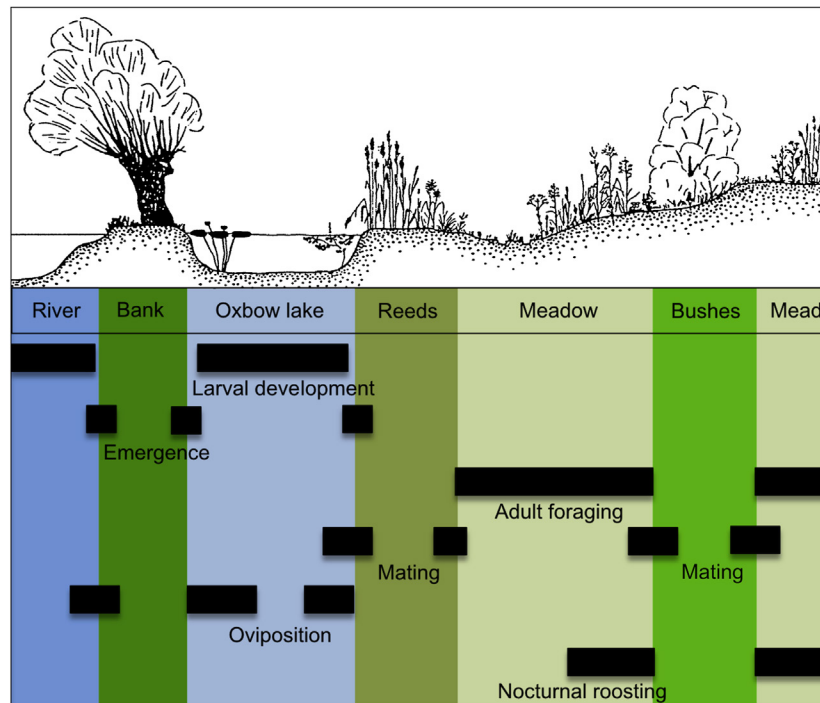
FIGURE 35.21 Use of various structures within the habitat, here a river floodplain, during successive stages in the life cycle of Platynemis pennipes (Pallas, 1771). Altered and redrawn from Martens (1996), with permission.
