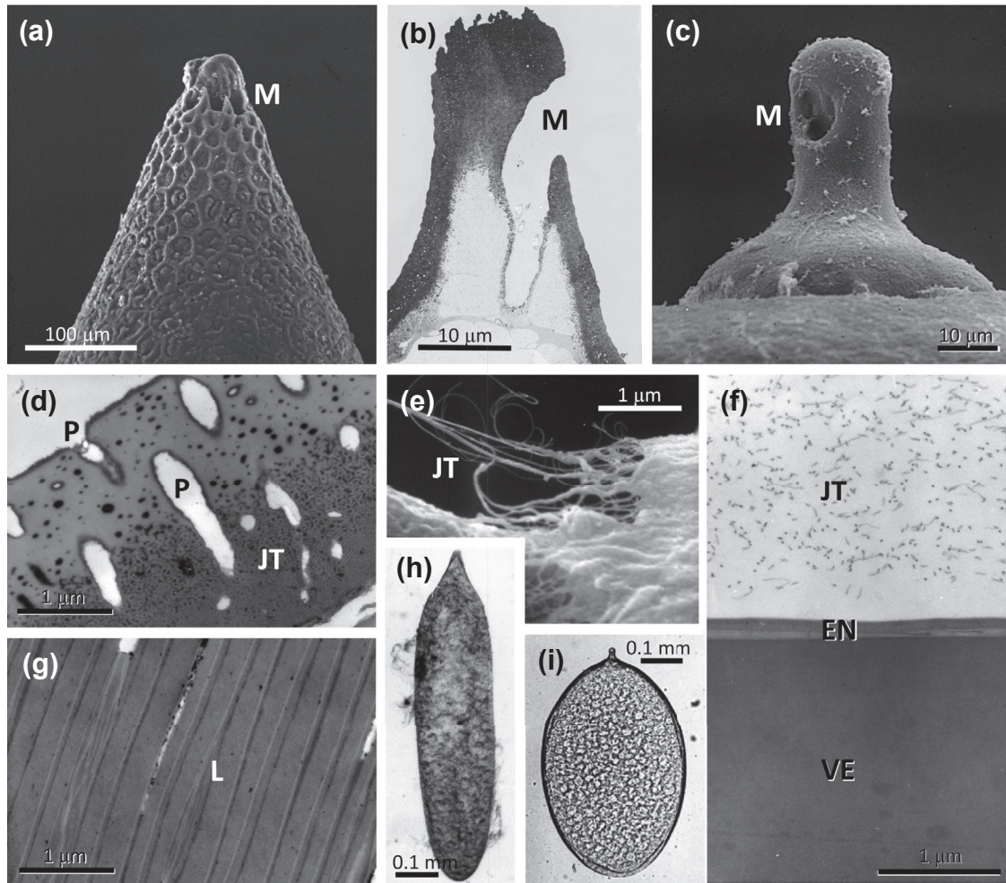
FIGURE 35.6 Eggs and egg shell details: (a) anterior end of endophytic eggshell in Aeshna juncea (Linnaeus, 1758); (b) anterior end of exophytic eggshell in Somatochlora metallica (Vander Linden, 1825), in cross section and (c) lateral view; (d) exochorion of A. juncea in cross-section; (e) jelly strands of S. metallica ; (f) cross-section of eggshell in Orthetrum cancellatum (Linnaeus, 1758); (g) endochorion of A. juncea in cross-section; (h) egg of Ischnura elegans (Vander Linden, 1820); and (i) egg of Somatochlora metallica (Vander Linden, 1825) (all new or adapted originals). EN, endochorion; JT, exochorionic jelly threads; L, lamellar layers; M, micropyle; P, exochorionic pores; VE, vitelline envelope. Photos by GS.
