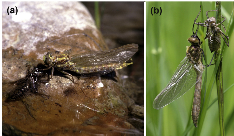
FIGURE 35.18 Freshly emerged Odonata sitting on the respective exuviae. Left: type 1 emergence of the gomphid Onychogomphus uncatius ; right: type 2 emergence of the corduliid Cordulia aenea (Linnaeus, 1758). Photos FS.
