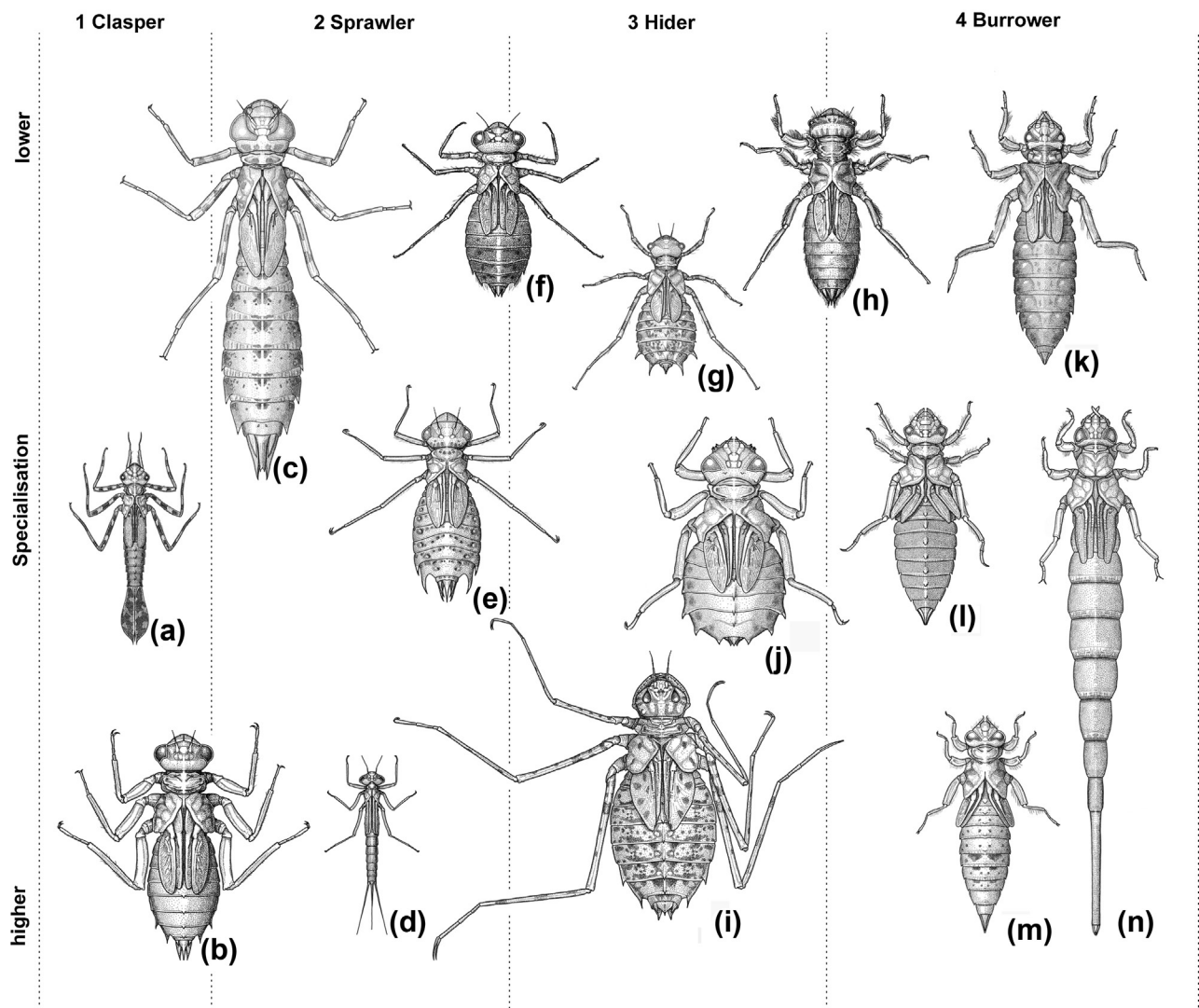
FIGURE 35.22 Body shapes and microhabitat types among Odonata. The graphic indicates the position of various body shapes along a gradient from clasper to sprawler, hider, and finally burrower. Drawings on the lines imply an intermediate position. (a) Umma (Calopterygidae); (b) Zygonyx (Libellulidae); (c) Anax (Aeshnidae); (d) Ischnura (Coenagrionidae); (e) Pantala Hagen, 1861; (f) Diplacodes Kirby, 1889; (g) Brachythemis Brauer, 1868; (h) Orthetrum (e–h Libellulidae); (i) Phyllomacromia (Macromiidae); (j) Gomphidia Selys, 1854; (k) Notogomphus Hagen, 1858; (l) Onychogomphus Selys, 1854; (m) Paragomphus ; and (n) Neurogomphus Karsch, 1890 (j–n Gomphidae). Drawings by Ole Müller.
