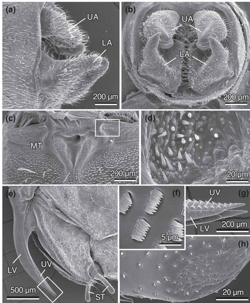
FIGURE 35.10 Details of some genital structure in dragonflies (SEM images). (a, b) Male upper (UA) and lower (LA) anal appendages in lateral view (a) of Enallagma ambiguum Navas, 1936, and posterior aspect (b) of E. risi Schmidt, 1961; (c, d) dorsal view of the mesothorax of the E. ambiguum female; this region is the attachment site for the male anal appendages and is richly equipped with trichoid sensilla; the white rectangle region (c) is also shown (d) enlarged; and (e–h) female abdominal structures in Calopteryx splendens showing typical endophytic ovipositor (e) with upper (UV) and lower valves (LV) and stylus (ST) in lateral aspect; the white rectangle region in (e) is also shown enlarged (g); (f) inner surface of the lower valvula covered with comb-like arrays of distally oriented microtrichia used for egg transport into plant tissues; the tip of the stylus (h) is richly equipped with numerous sensilla. Photos by SG.
