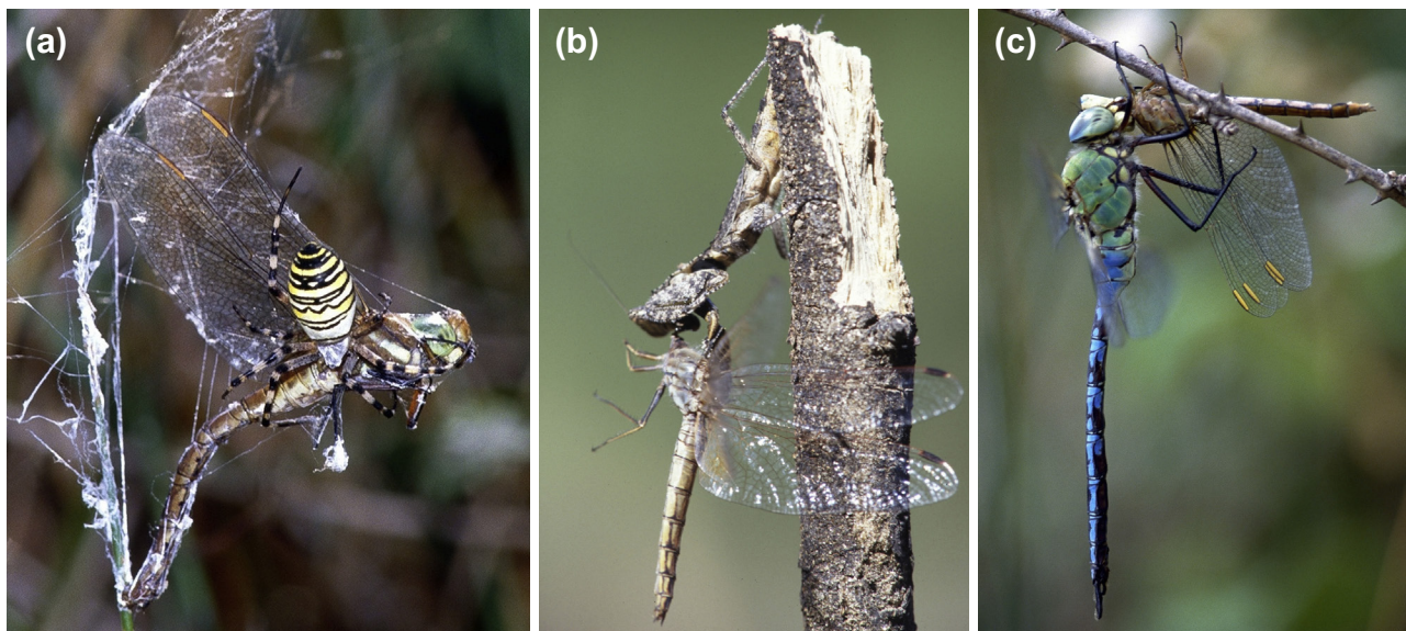
FIGURE 35.23 Predators of adult dragonflies. (a) Aeshna isoceles (Müller, 1776), caught in the web of spider, Argiope bruennichi (Scopoli, 1772); (b) Trithemis kirbyi Selys, 1891, female caught by a mantid, probably of the genus Tarachodes ; and (c) immature Orthetrum coerulescens (Fabricius, 1798), caught during maiden flight by another dragonfly, Anax imperator . Photos by FS.
